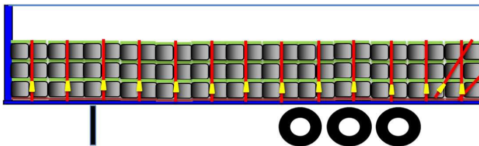
13 over the top straps applied to the whole load
