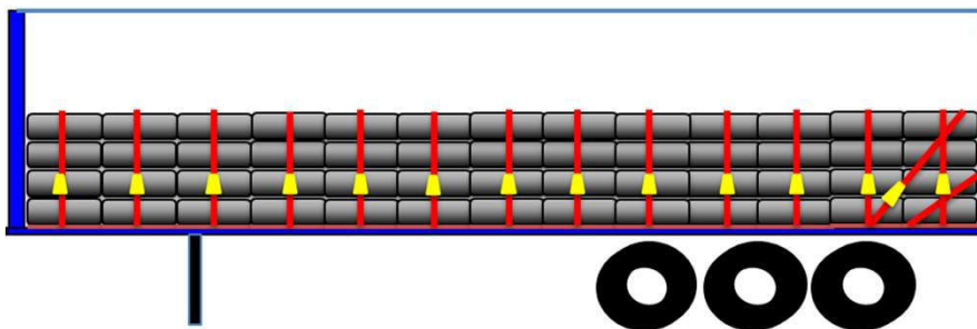
13 over the top straps applied to the whole load
