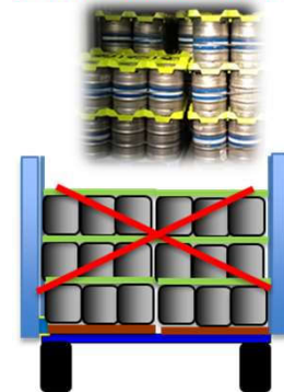
2 straps applied in a cross over rear pallets
